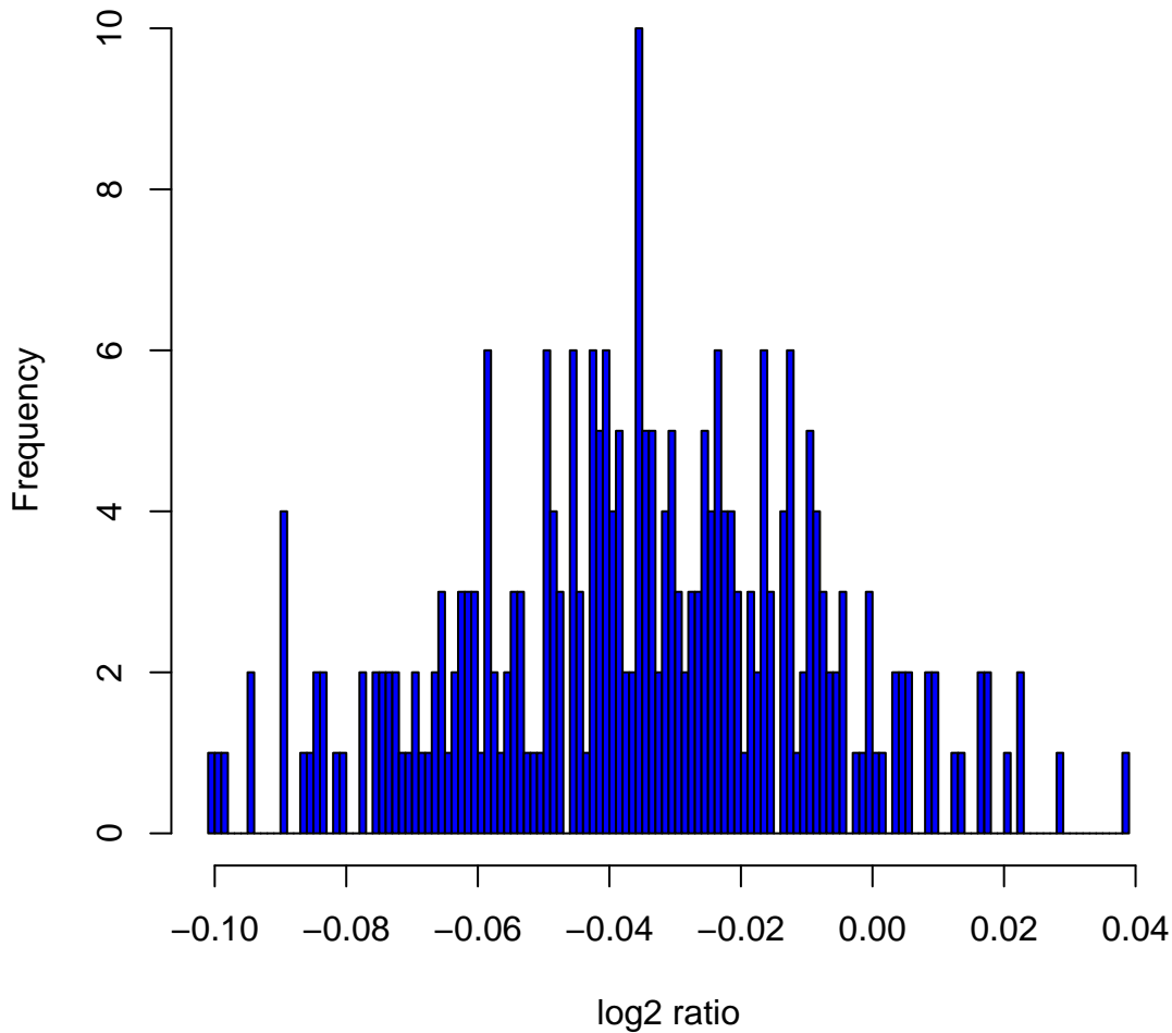
Histogram of log 2 ratios in 270 HapMap samples at clone Chr3tp-4B8
