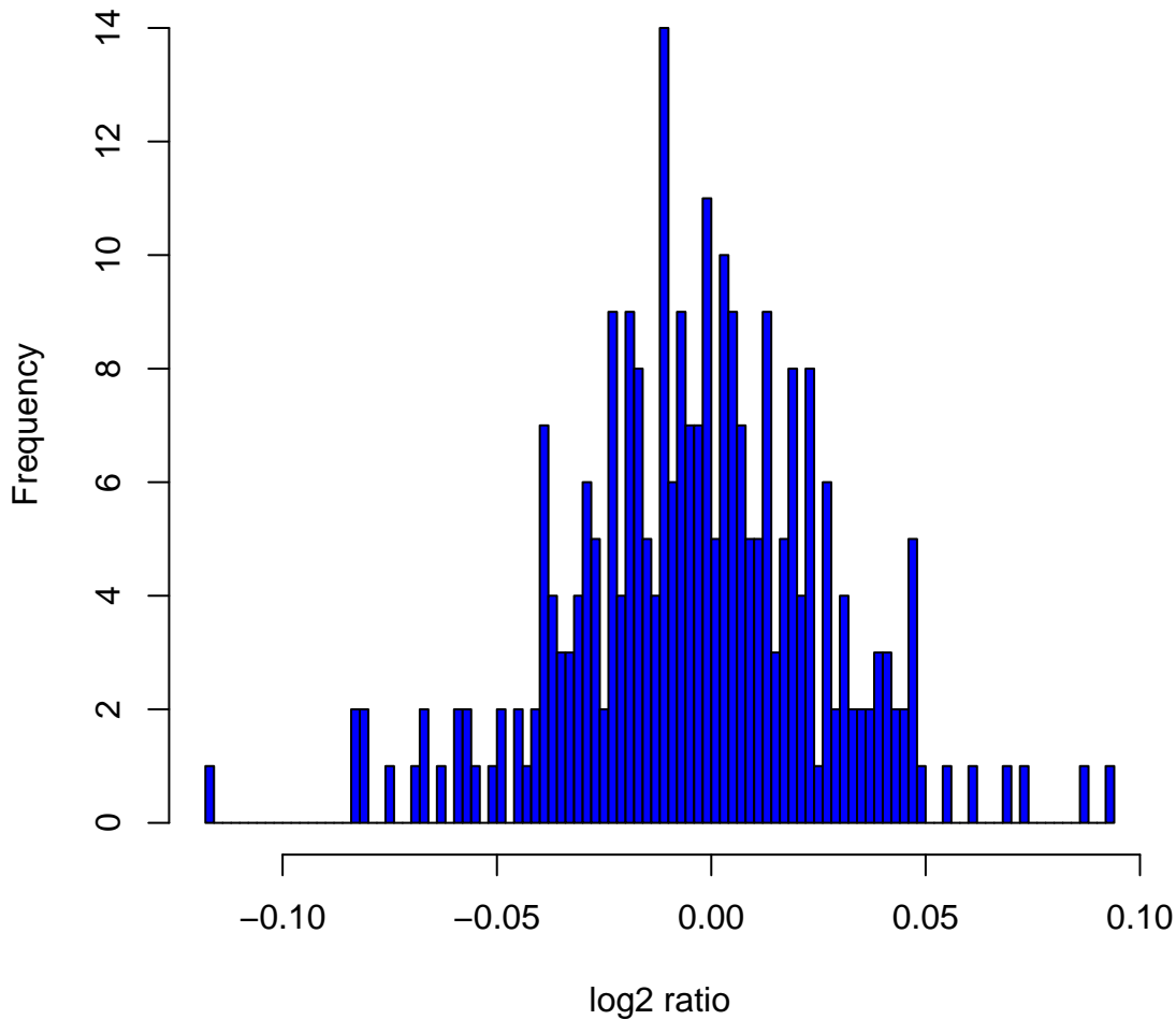
Histogram of log2ratios in 270 HapMap samples at clone Chr3tp-4E2
