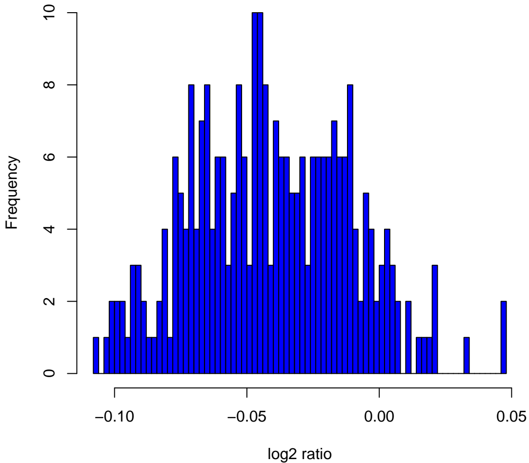
Histogram of log2ratios in 270 HapMap samples at clone Chr3tp-4H4
