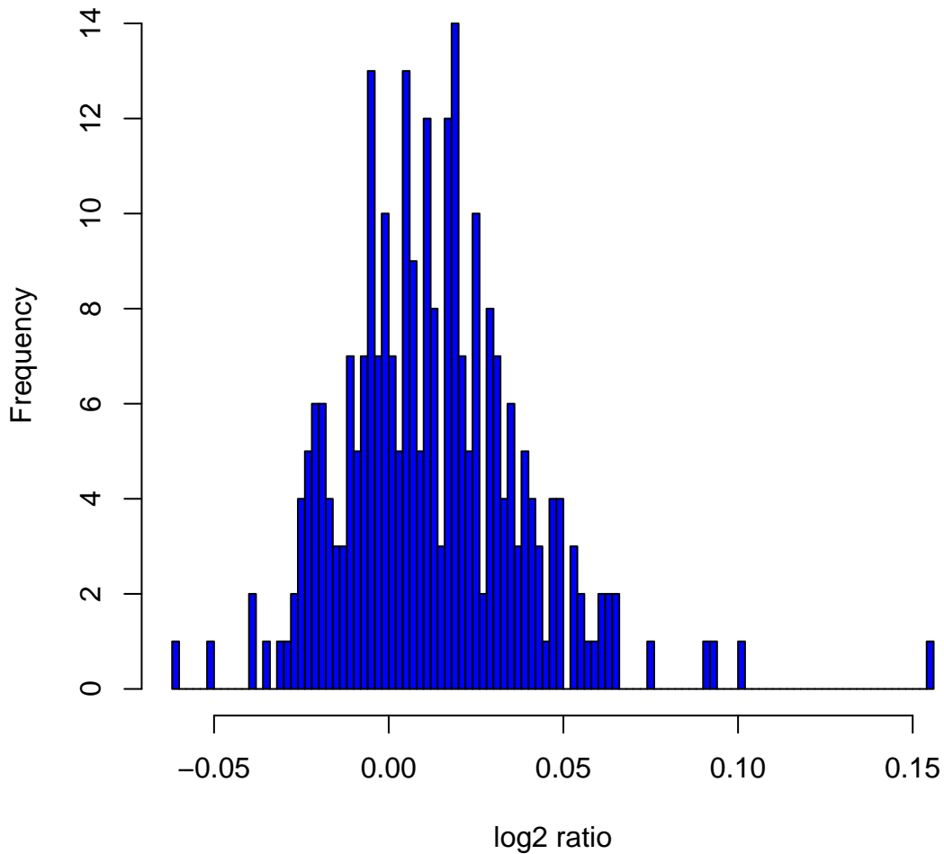
Histogram of log 2 ratios in 270 HapMap samples at clone Chr3tp-4H6
