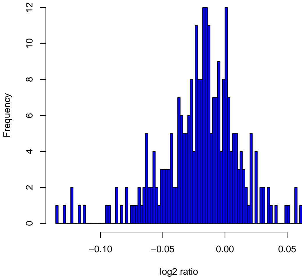
Histogram of \log_2 ratios in 270 HapMap samples at clone Chr3tp-5A1
