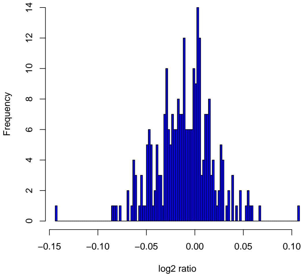
Histogram of log 2 ratios in 270 HapMap samples at clone Chr3tp-5A7
