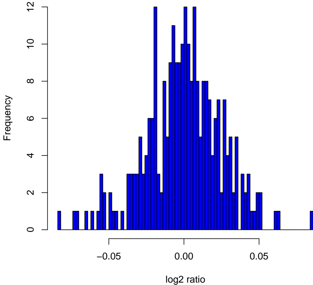
Histogram of log 2 ratios in 270 HapMap samples at clone Chr3tp-5B12
