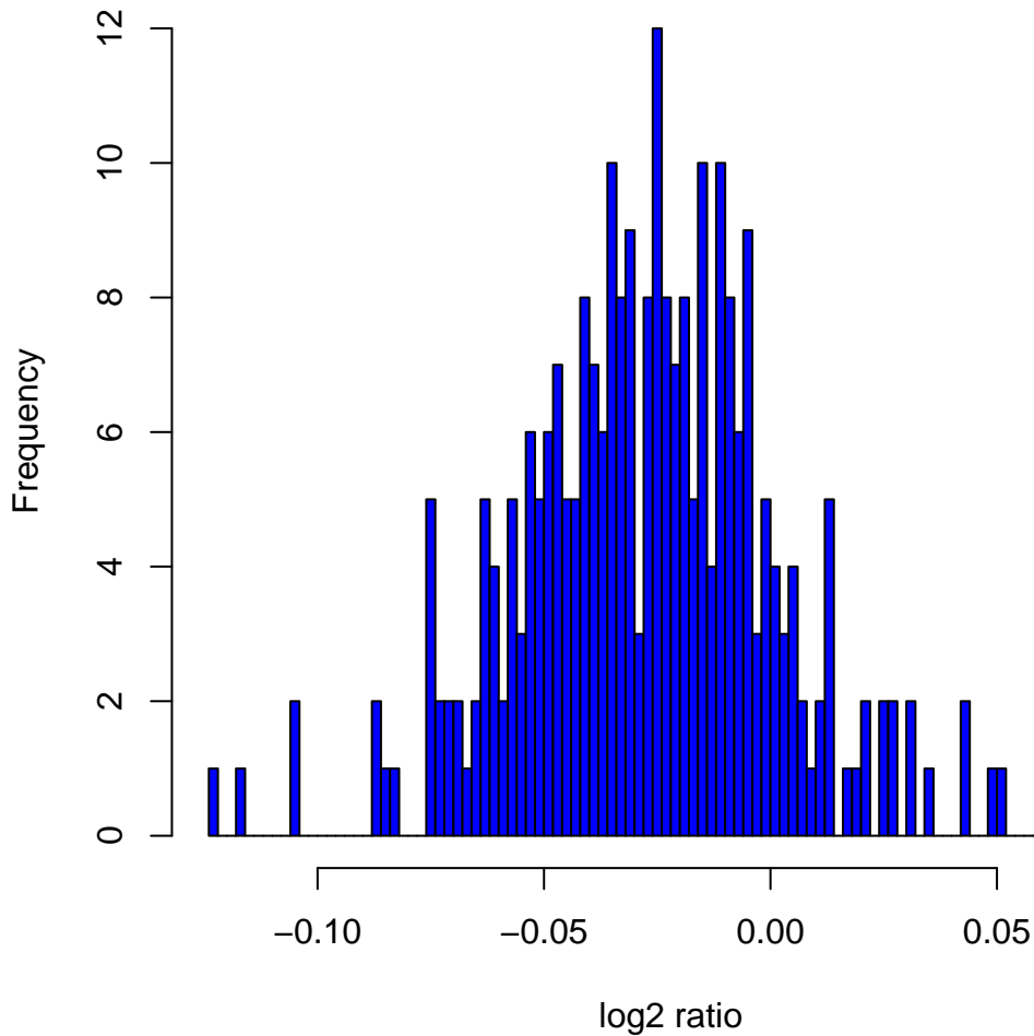
Histogram of log 2 ratios in 270 HapMap samples at clone Chr3tp-5B2
