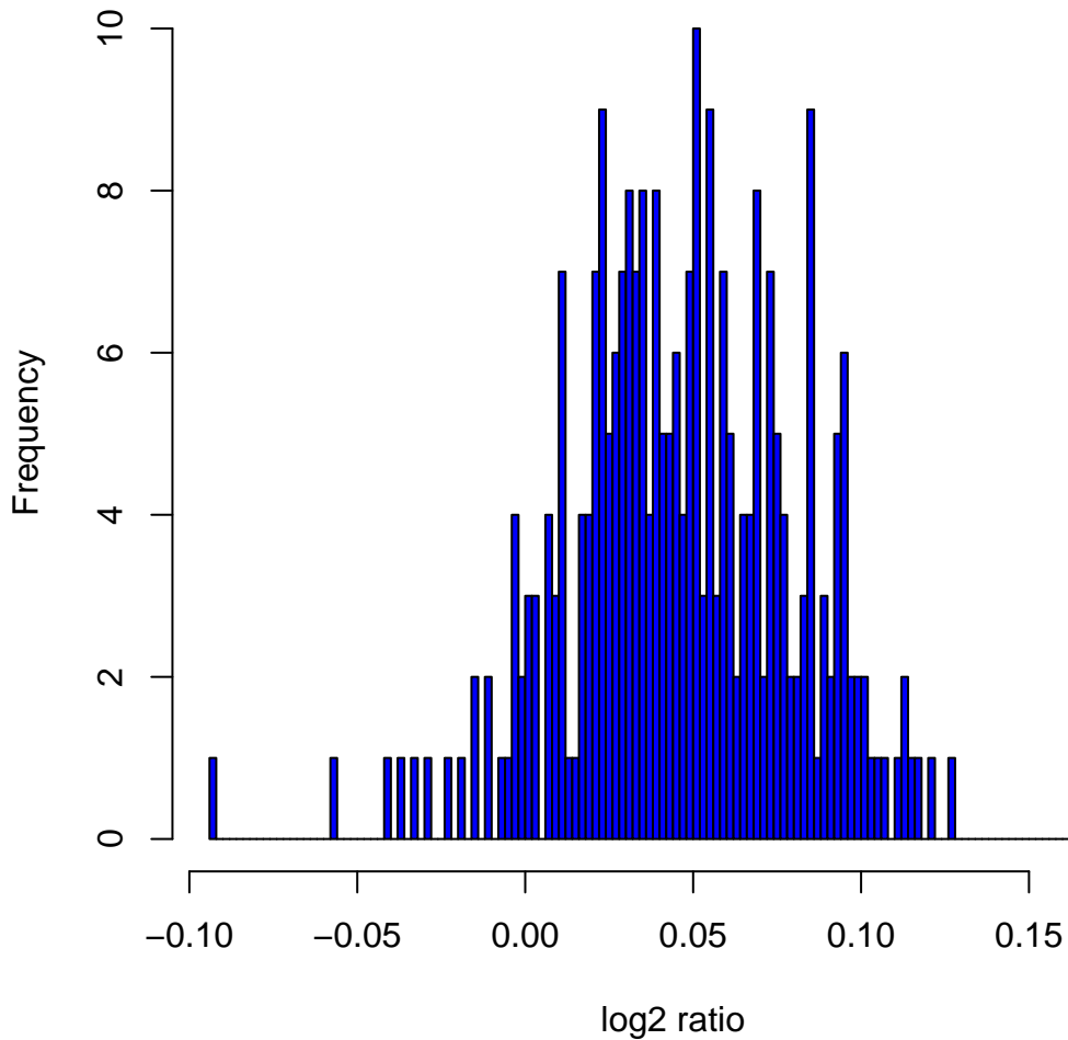
Histogram of \log_2 ratios in 270 HapMap samples at clone Chr3tp-5B5
