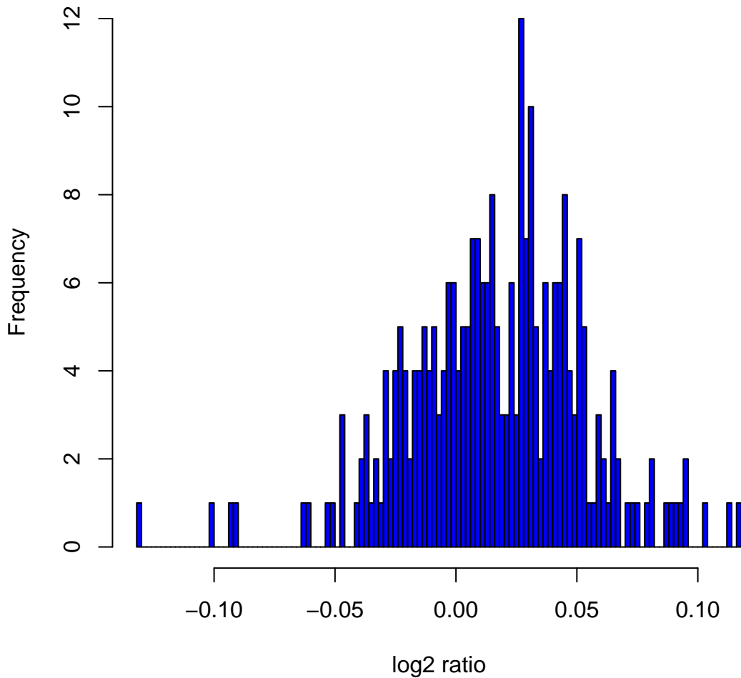
Histogram of \log_2 ratios in 270 HapMap samples at clone Chr3tp-5D1
