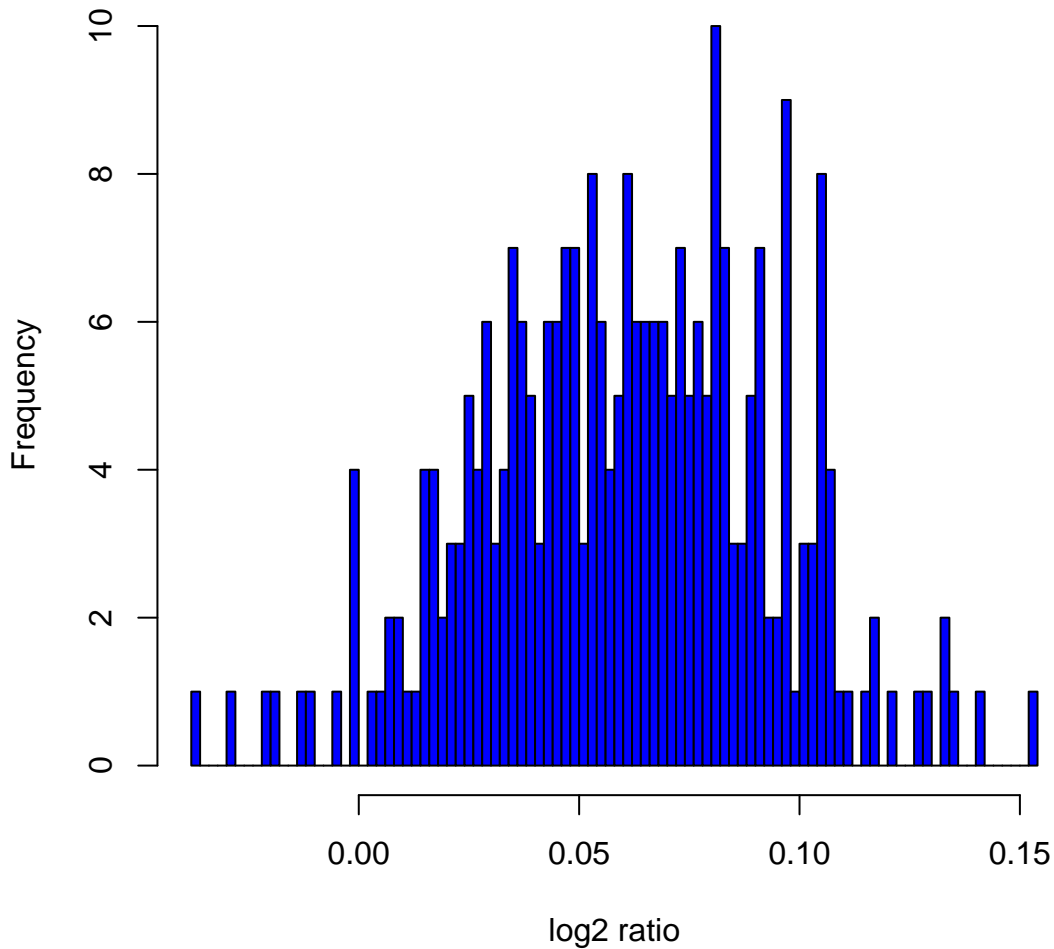
Histogram of log 2 ratios in 270 HapMap samples at clone Chr3tp-5D9
