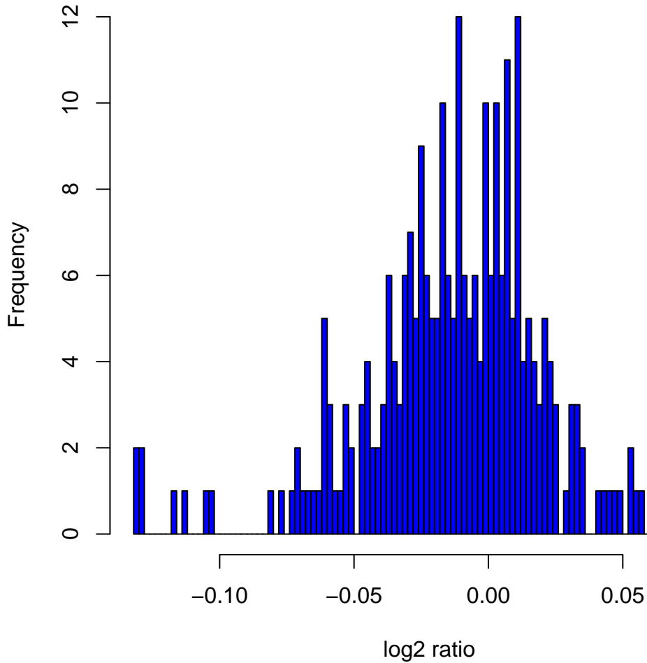
Histogram of log2ratios in 270 HapMap samples at clone Chr3tp-5F1
