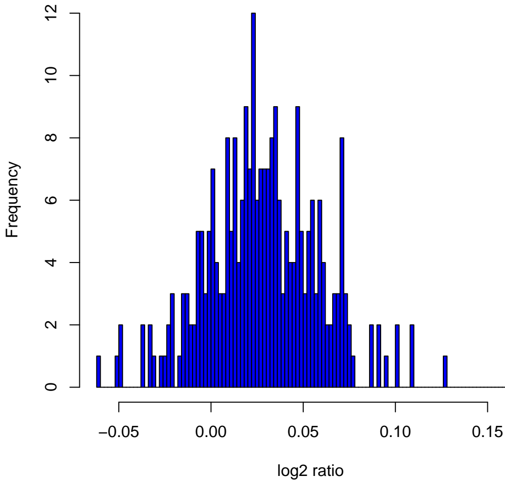
Histogram of log2ratios in 270 HapMap samples at clone Chr3tp-5F2
