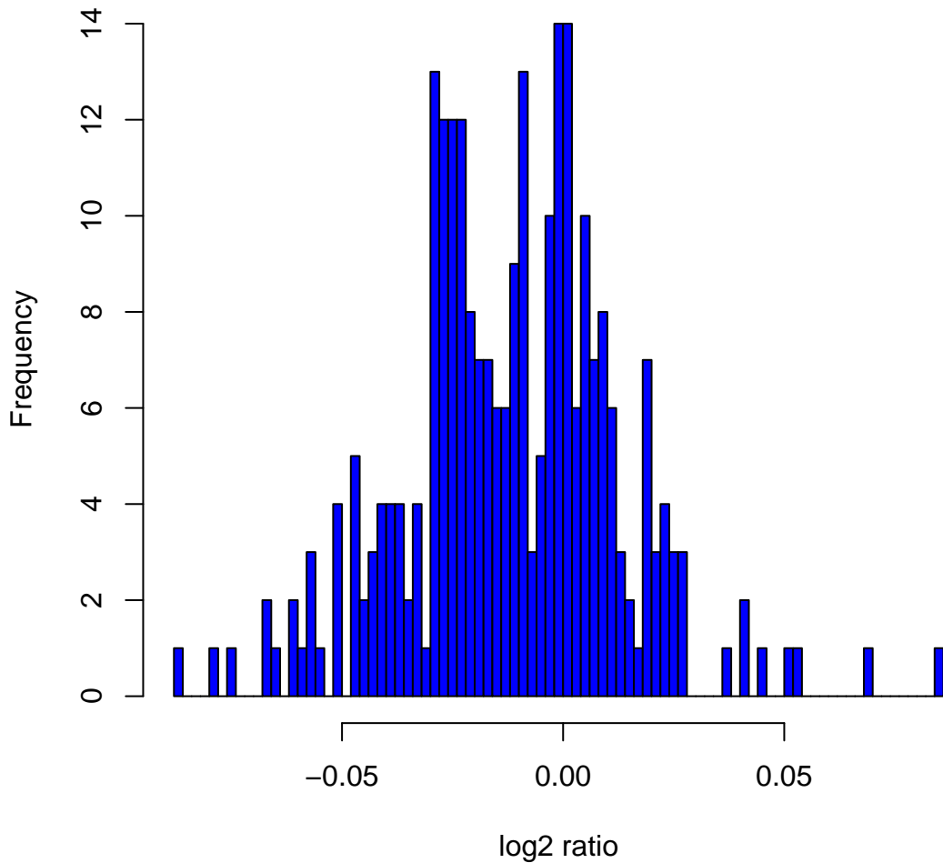
Histogram of \log_2 ratios in 270 HapMap samples at clone Chr3tp-5G11
