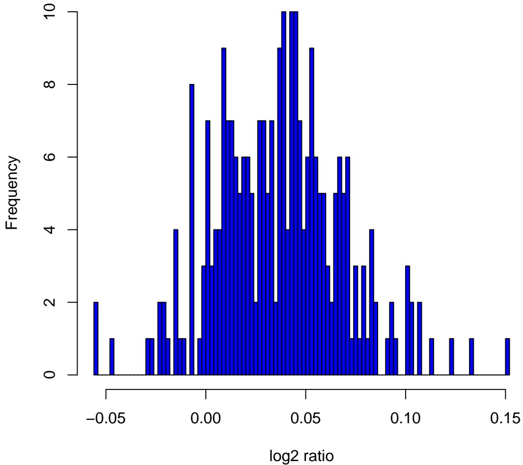
Histogram of \log_2 ratios in 270 HapMap samples at clone Chr3tp-5G12
