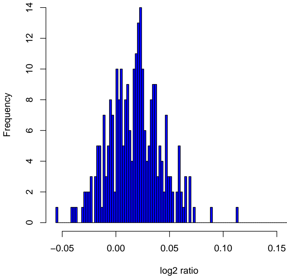
Histogram of \log_2 ratios in 270 HapMap samples at clone Chr3tp-5G2
