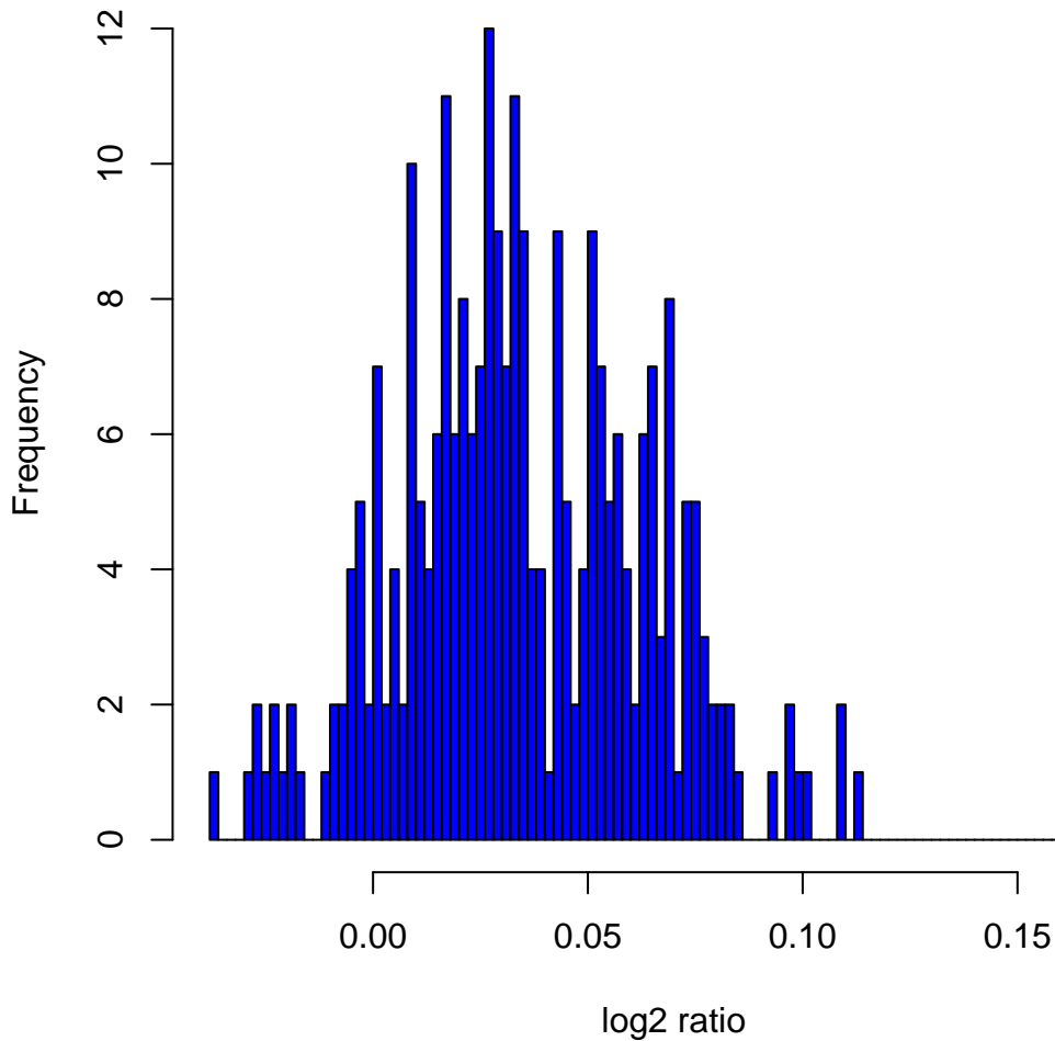
Histogram of log2ratios in 270 HapMap samples at clone Chr3tp-5G7
