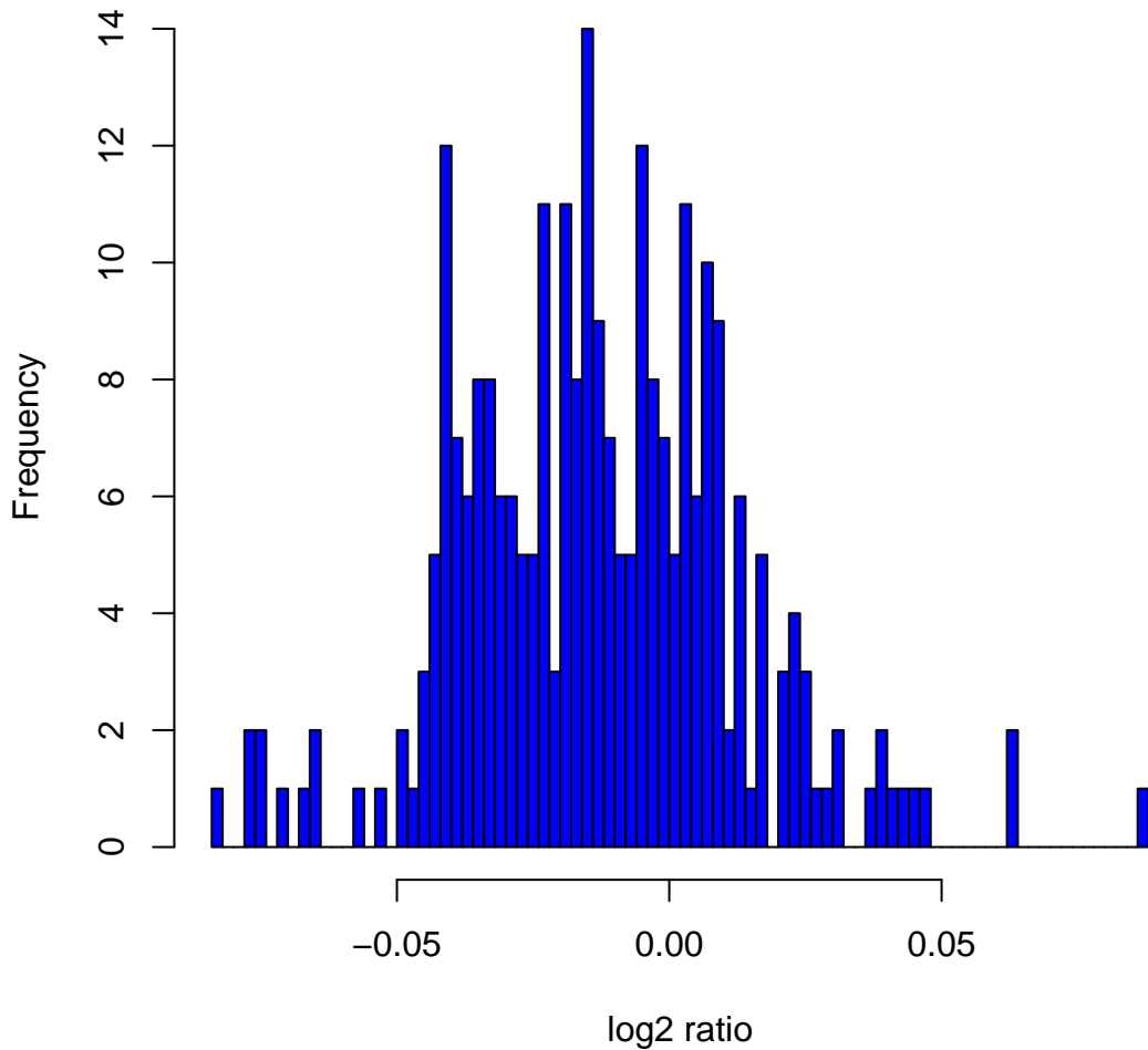
Histogram of log 2 ratios in 270 HapMap samples at clone Chr3tp-5H3
