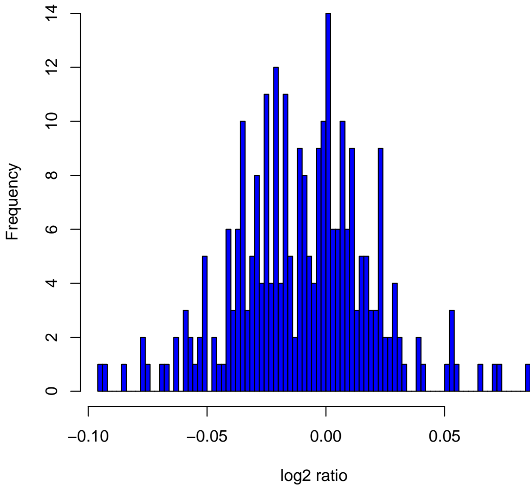
Histogram of log 2 ratios in 270 HapMap samples at clone Chr3tp-6A1
