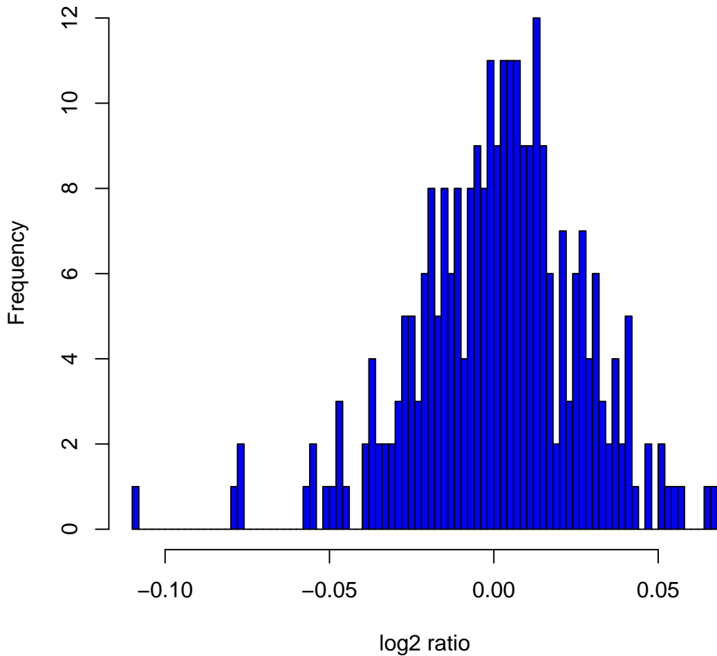
Histogram of log 2 ratios in 270 HapMap samples at clone Chr3tp-6A3
