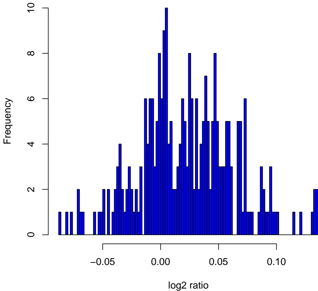
Histogram of \log_2 ratios in 270 HapMap samples at clone Chr3tp-6A4
