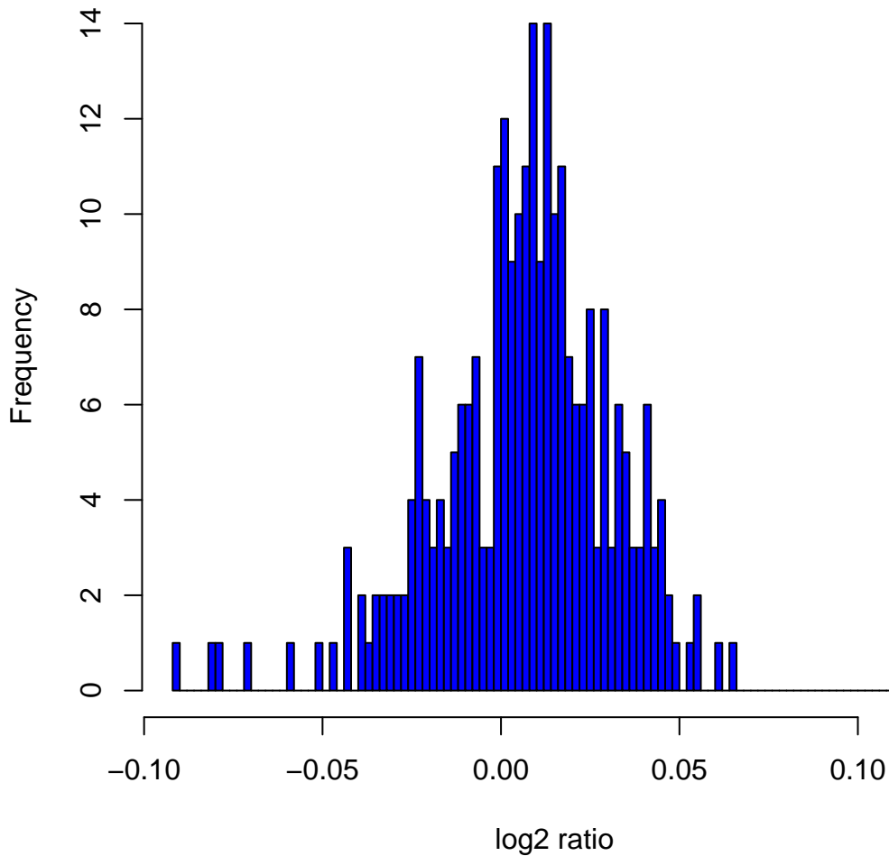
Histogram of \log_2 ratios in 270 HapMap samples at clone Chr3tp-6A5
