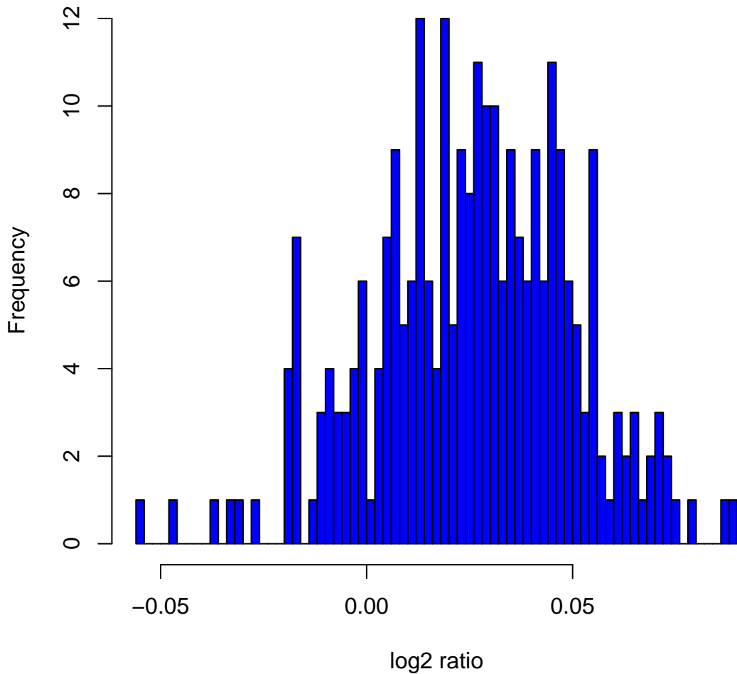
Histogram of log 2 ratios in 270 HapMap samples at clone Chr3tp-6A8
