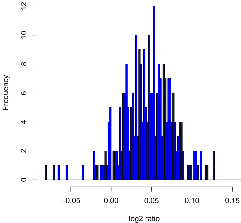
Histogram of \log_2 ratios in 270 HapMap samples at clone Chr3tp-6A9
