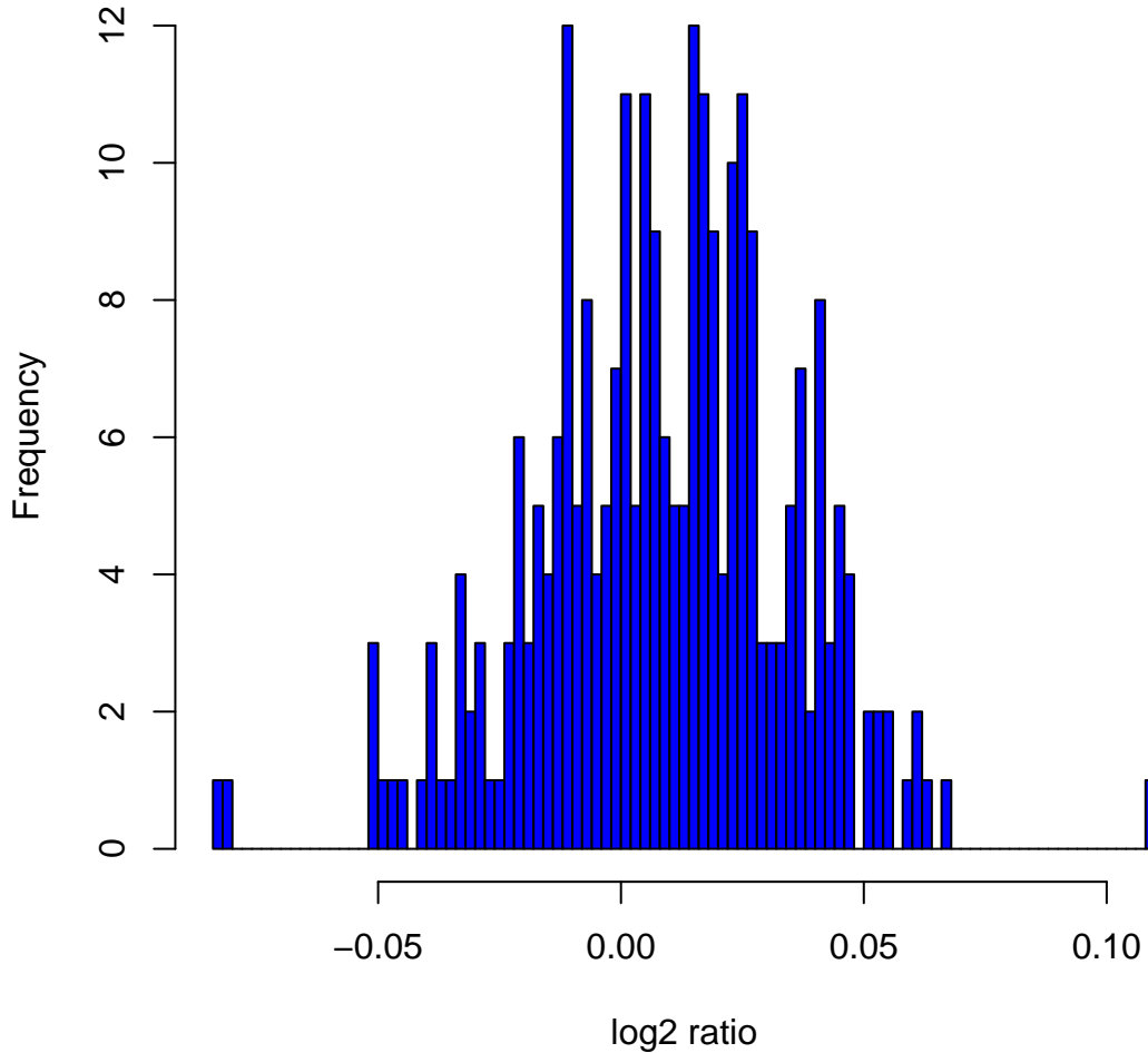
Histogram of log2ratios in 270 HapMap samples at clone Chr3tp-6B11
