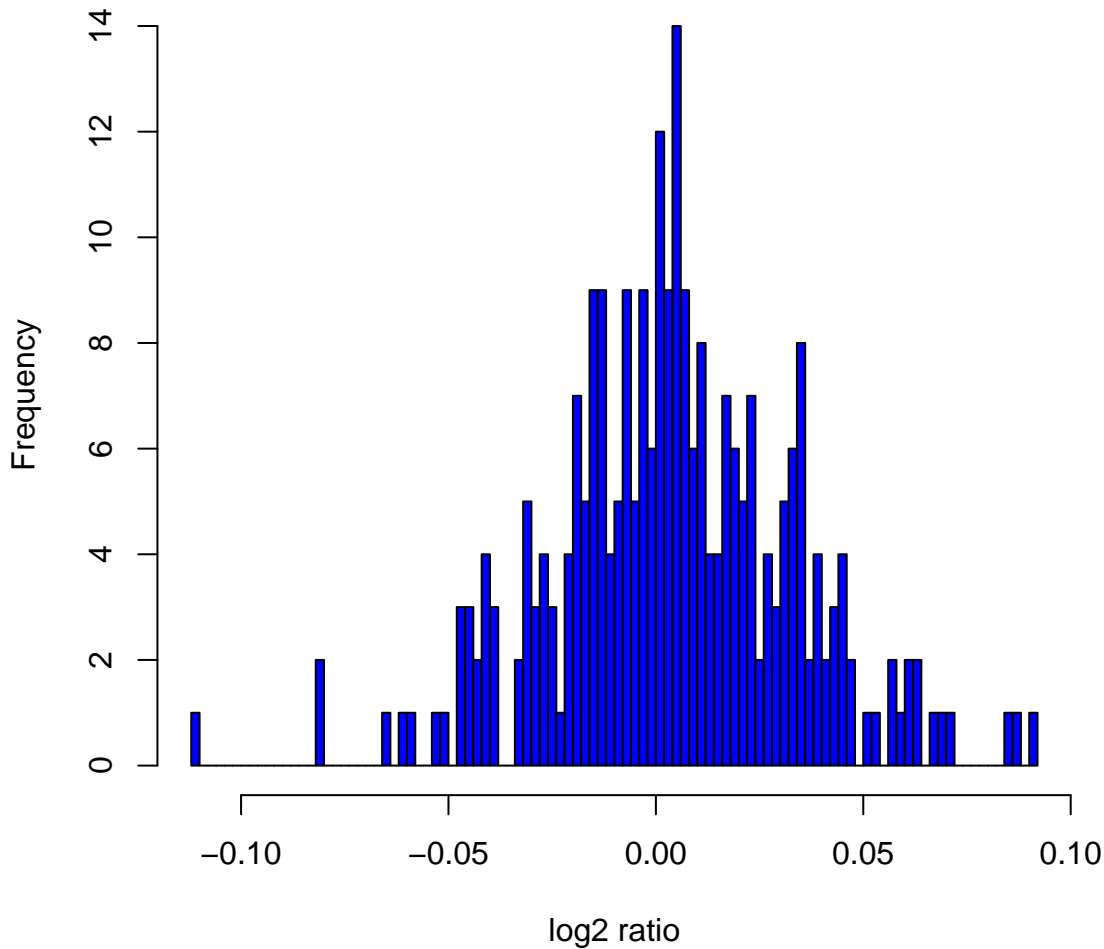
Histogram of log 2 ratios in 270 HapMap samples at clone Chr3tp-6B2
