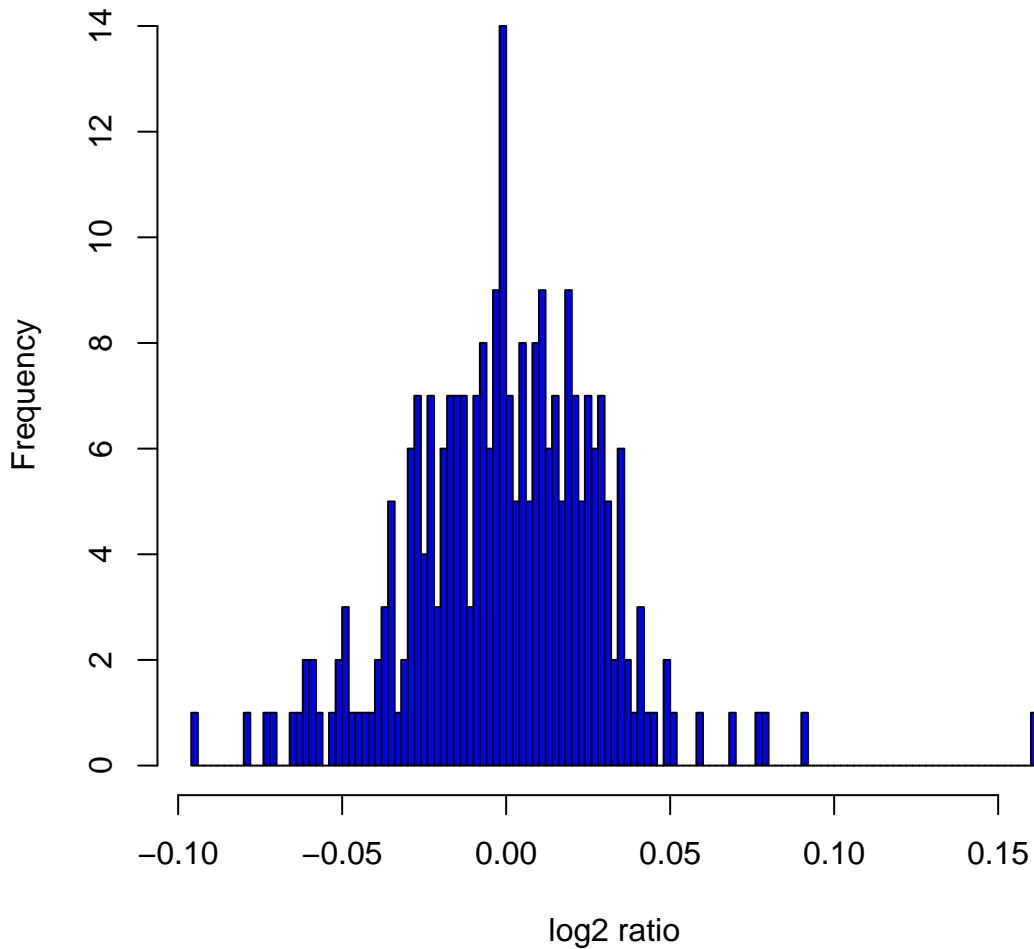
Histogram of log 2 ratios in 270 HapMap samples at clone Chr3tp-6B4
