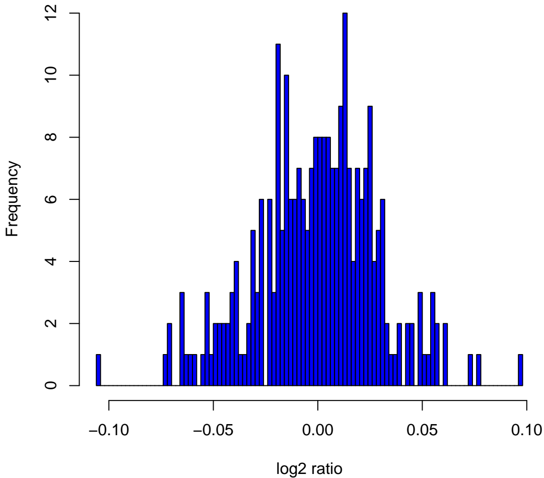
Histogram of log 2 ratios in 270 HapMap samples at clone Chr3tp-6C1
