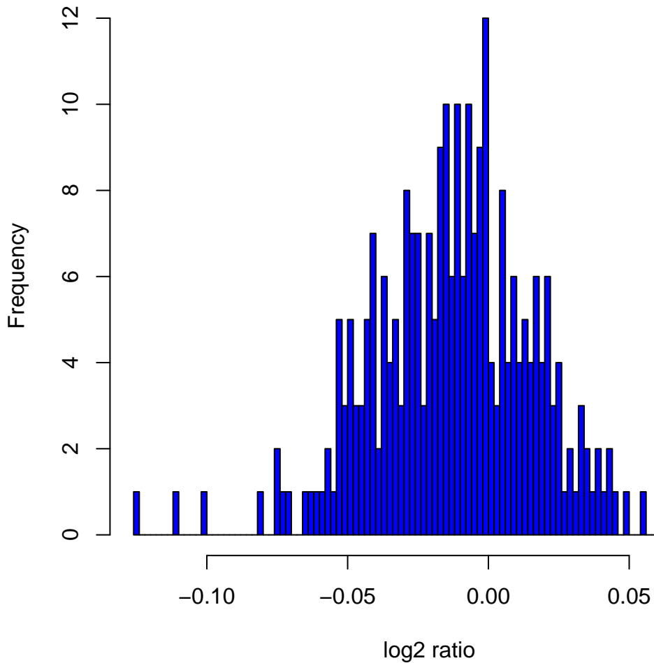
Histogram of \log_2 ratios in 270 HapMap samples at clone Chr3tp-6C5
