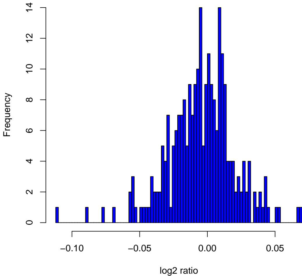
Histogram of log2ratios in 270 HapMap samples at clone Chr3tp-6D11
