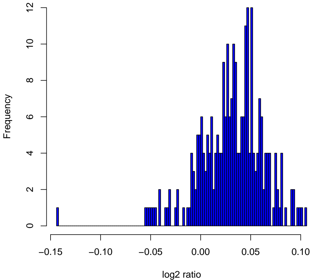
Histogram of log 2 ratios in 270 HapMap samples at clone Chr3tp-6D5
