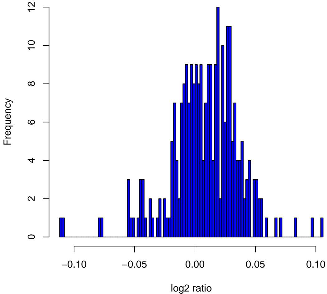
Histogram of log2ratios in 270 HapMap samples at clone Chr3tp-6F1
