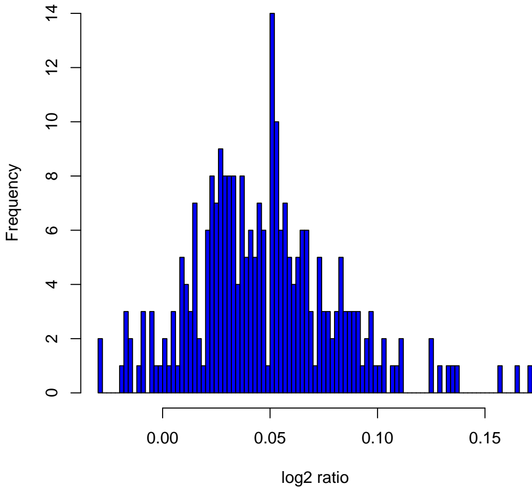
Histogram of log2ratios in 270 HapMap samples at clone Chr3tp-6G1
