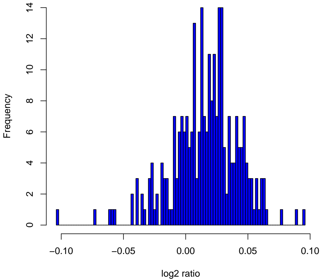
Histogram of log 2 ratios in 270 HapMap samples at clone Chr3tp-6G2
