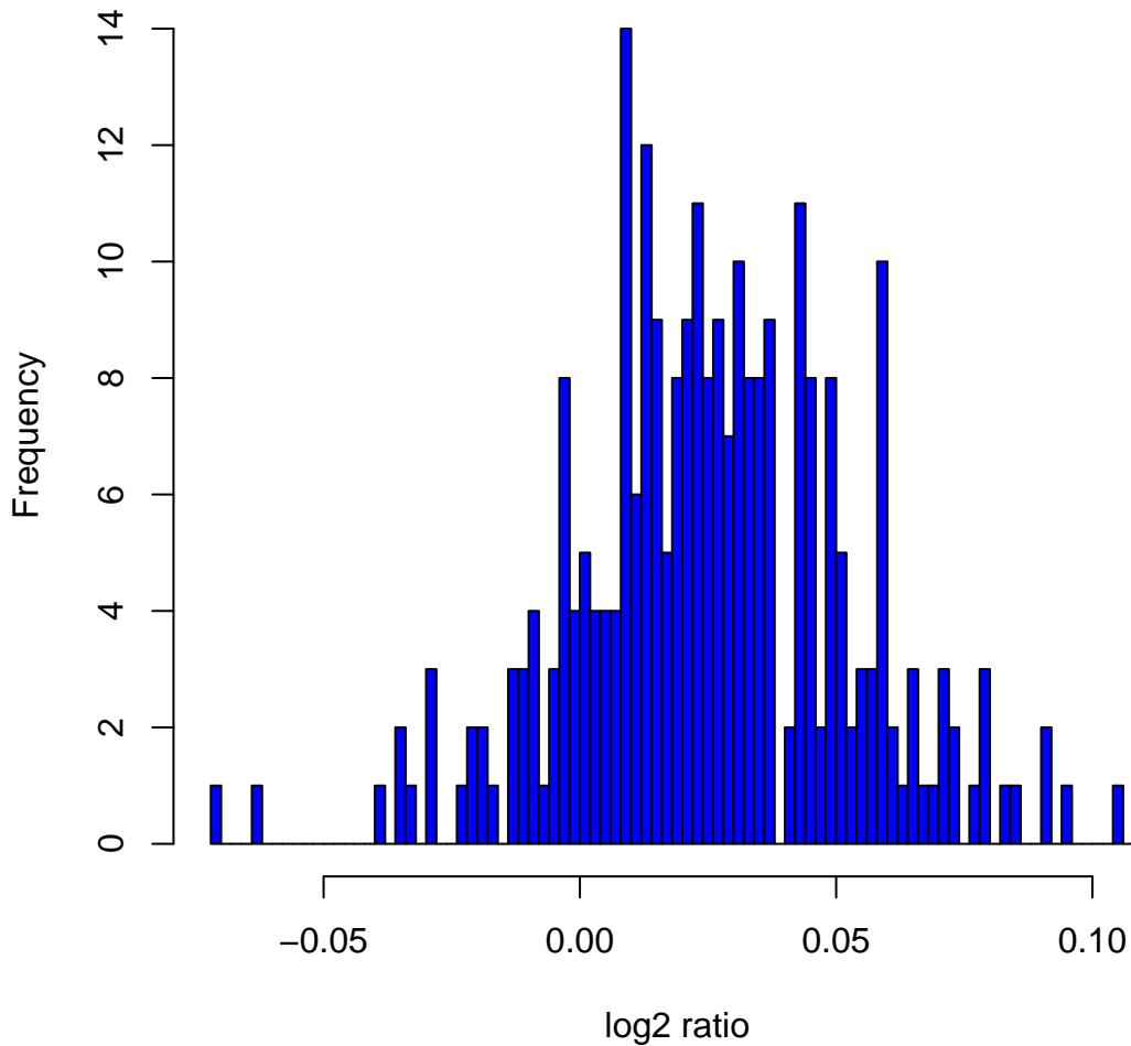
Histogram of \log_2 ratios in 270 HapMap samples at clone Chr3tp-6G3
