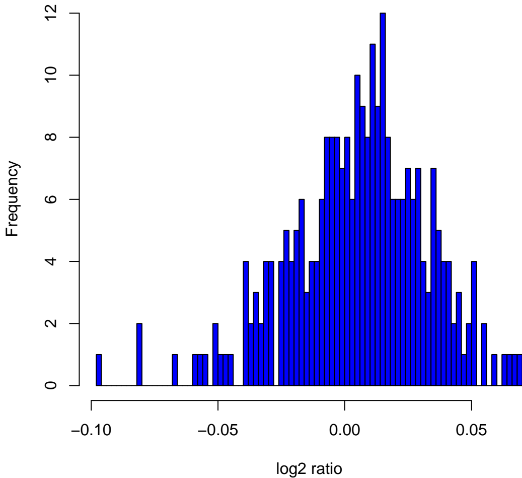
Histogram of \log_2 ratios in 270 HapMap samples at clone Chr3tp-6G7
