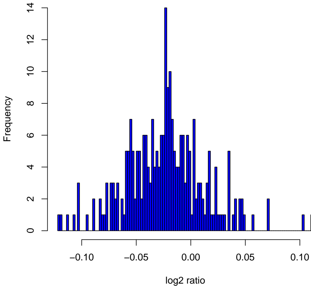
Histogram of log 2 ratios in 270 HapMap samples at clone Chr3tp-6H1
