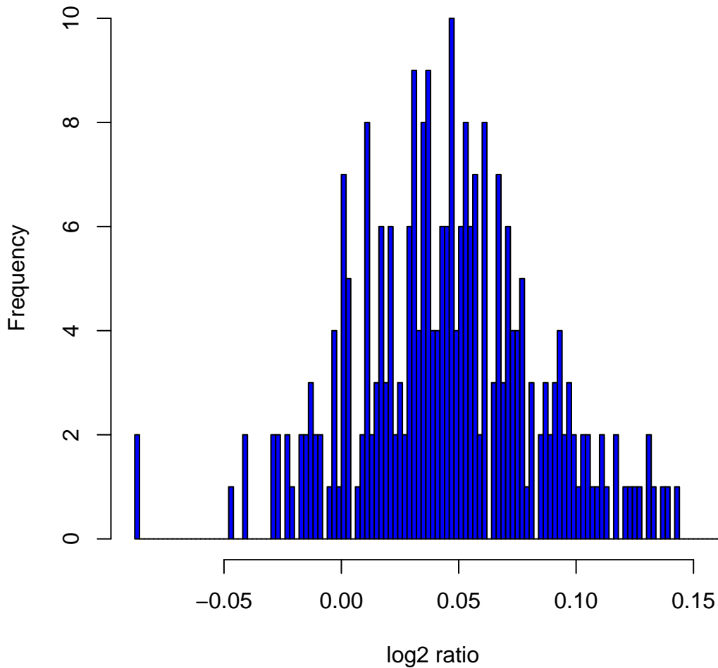
Histogram of log 2 ratios in 270 HapMap samples at clone Chr3tp-6H3
