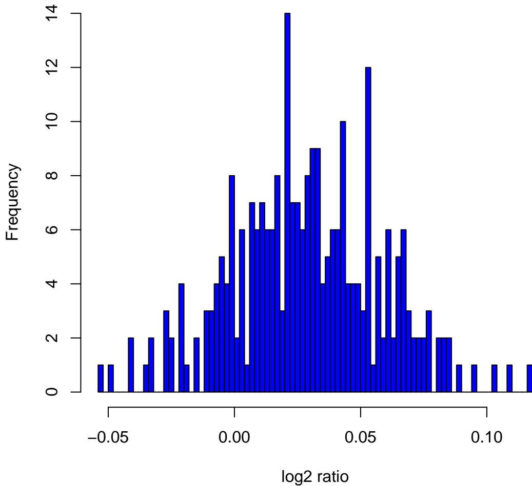
Histogram of log 2 ratios in 270 HapMap samples at clone Chr3tp-7A1
