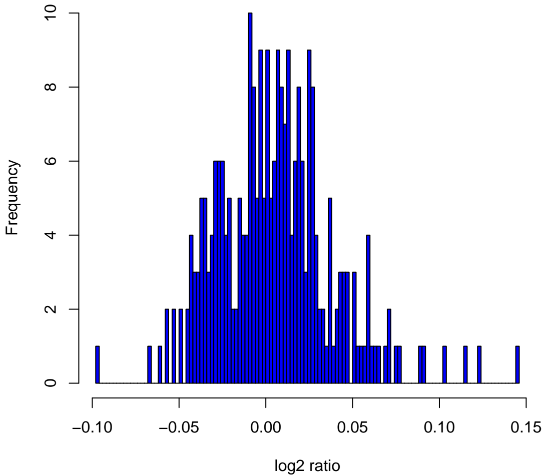
Histogram of log 2 ratios in 270 HapMap samples at clone Chr3tp-7B9
