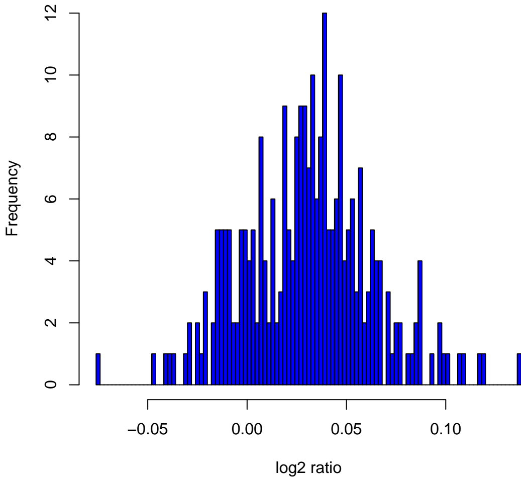
Histogram of \log_2 ratios in 270 HapMap samples at clone Chr3tp-7D8
