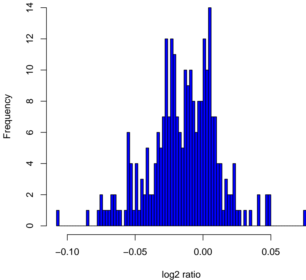
Histogram of log 2 ratios in 270 HapMap samples at clone Chr3tp-7F10
