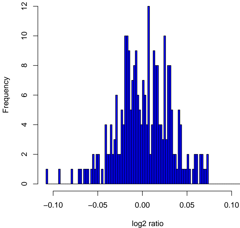
Histogram of log2ratios in 270 HapMap samples at clone Chr3tp-7F3
