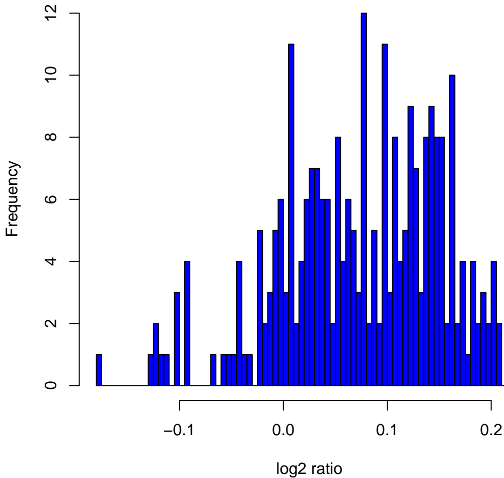
Histogram of log2ratios in 270 HapMap samples at clone Chr3tp-7F8
