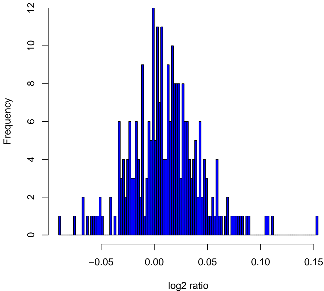
Histogram of \log_2 ratios in 270 HapMap samples at clone Chr3tp-7G7
