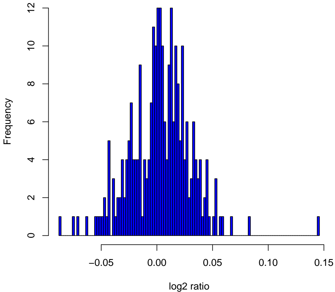
Histogram of \log_2 ratios in 270 HapMap samples at clone Chr3tp-7H7
