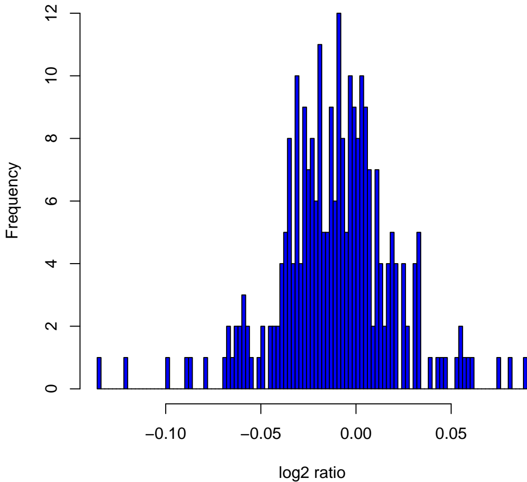
Histogram of log 2 ratios in 270 HapMap samples at clone Chr3tp-7H8
