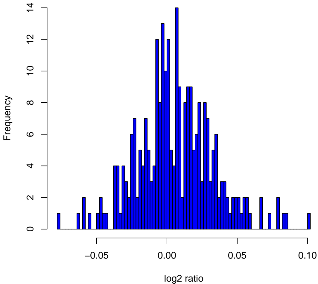
Histogram of log 2 ratios in 270 HapMap samples at clone Chr3tp-7H9
