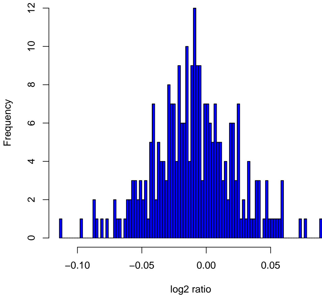
Histogram of log 2 ratios in 270 HapMap samples at clone Chr3tp-8A3
