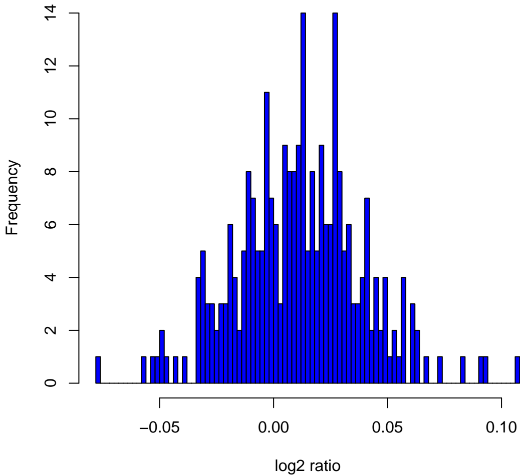
Histogram of log 2 ratios in 270 HapMap samples at clone Chr3tp-8A9
